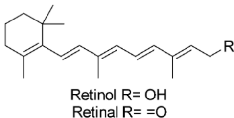
Figure 1: Structure of retinal and retinol
