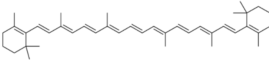
Figure 2: Structure of \beta -carotene
