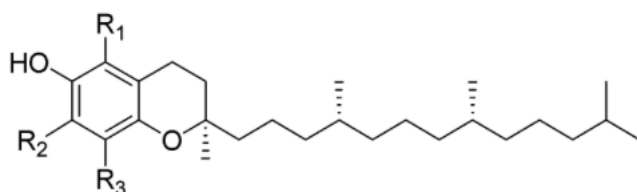
Figure 1: The tocopherol isomers \alpha : R_1 = CH_3 , R_2 = CH_3 , R_3 = CH_3 | \beta : R_1 = CH_3 , R_2 = H , R_3 = CH_3 | \gamma : R_1 = H , R_2 = CH_3 , R_3 = CH_3 | \delta : R_1 = H , R_2 = H , R_3 = CH_3
