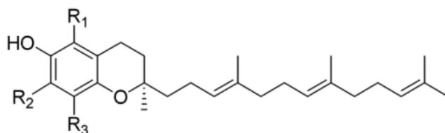
Figure 2: The tocotrienol isomers \alpha : R_1 = CH_3 , R_2 = CH_3 , R_3 = CH_3 | \beta : R_1 = CH_3 , R_2 = H , R_3 = CH_3 | \gamma : R_1 = H , R_2 = CH_3 , R_3 = CH_3 | \delta : R_1 = H , R_2 = H , R_3 = CH_3
